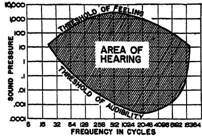
Threshold of audibility for average human ear. Shaded region is area of hearing.
